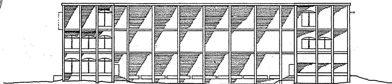
ELEVATION: B-B
