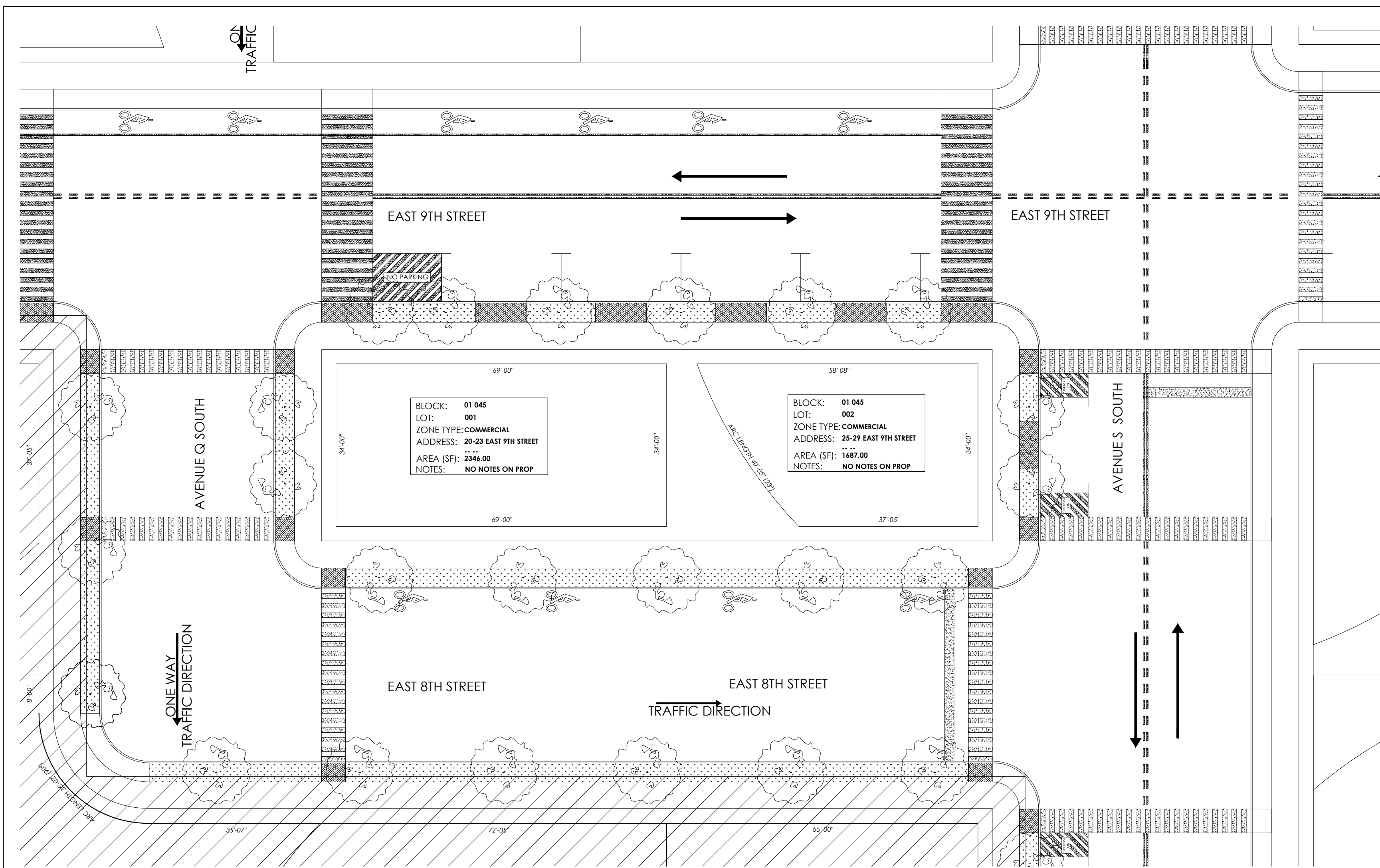
1 BLOCK PLAN BLOCK 01 045 G-004.94 SCALE: 1/16" = 1' - 0"
