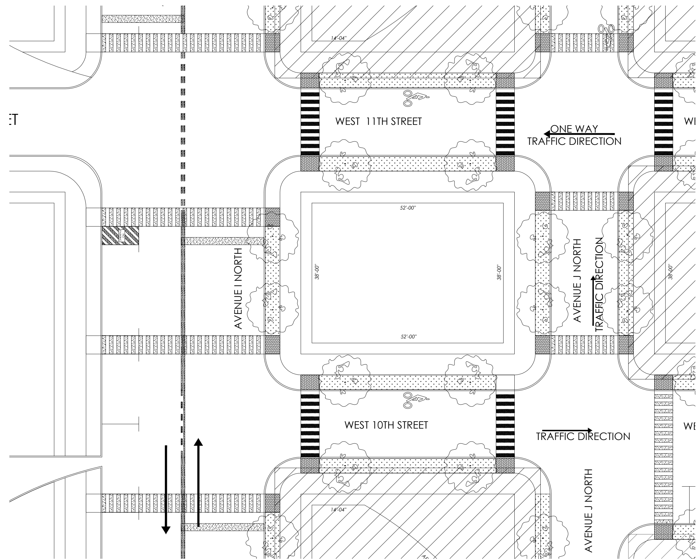
1 BLOCK 01 062 - PLAN G-004.132 SCALE: 1/16" = 1'-0"
