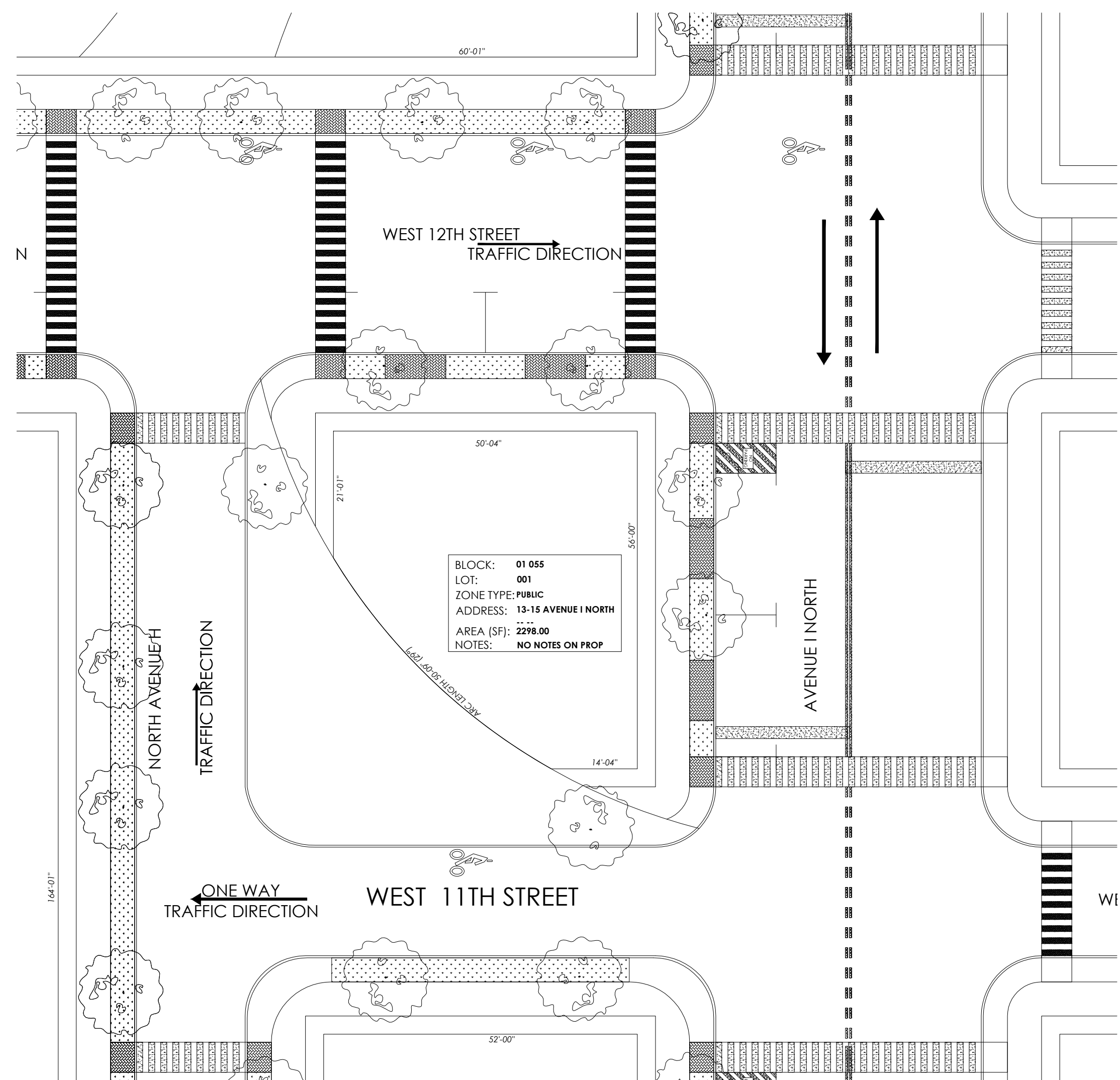
1 PHASE J NEIGHBORHOOD PLAN BLOCK 01 055 G-004.115 SCALE: 1/16" = 1'-0"
